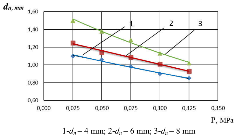
Figure 5. Dependence of the diameter of water droplets formed in the deflector nozzle on the water pressure in the nozzle tube.
