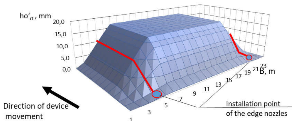
Figure 11. Water depth distribution curve produced by the device in a single pass.
