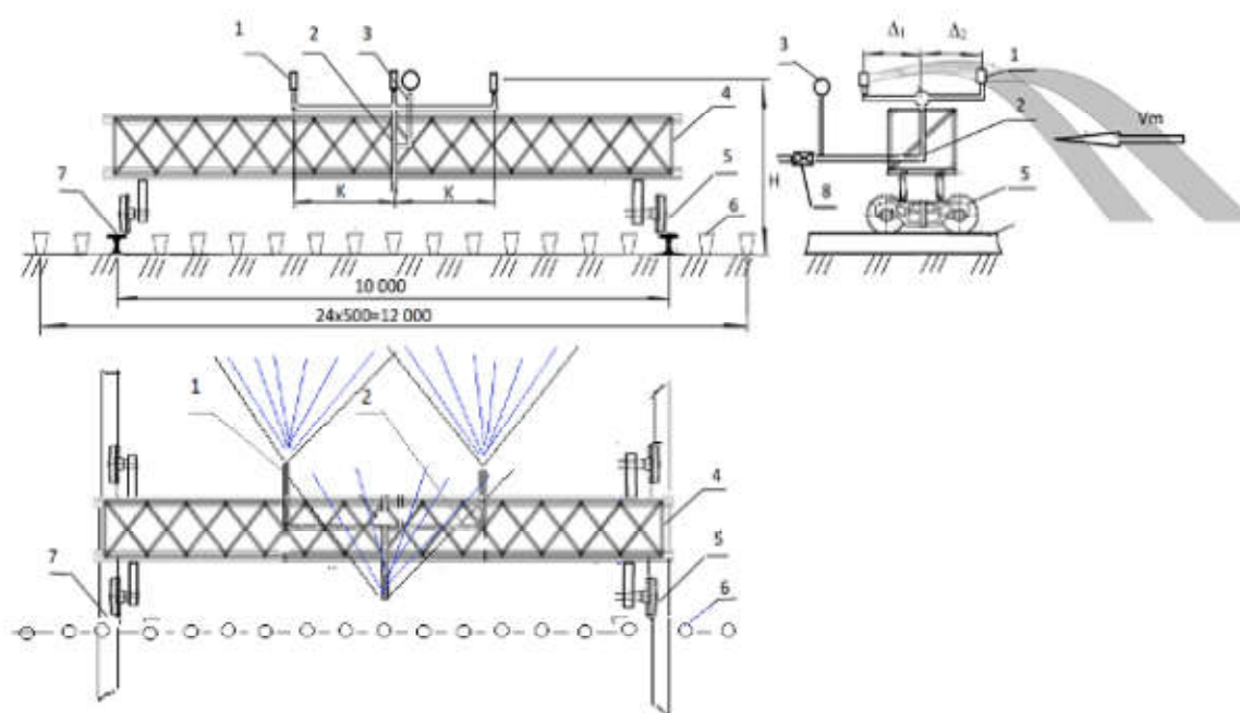
1 — sprinkler nozzle; 2 — water supply pipe; 3 — pressure gauge; 4 — test stand trolley; 5 — trolley wheel; 6 — rain gauges; 7 — rails.
