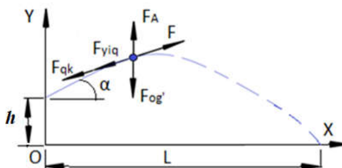
Figure 3. Main forces acting on a water droplet during the sprinkler irrigation process.
