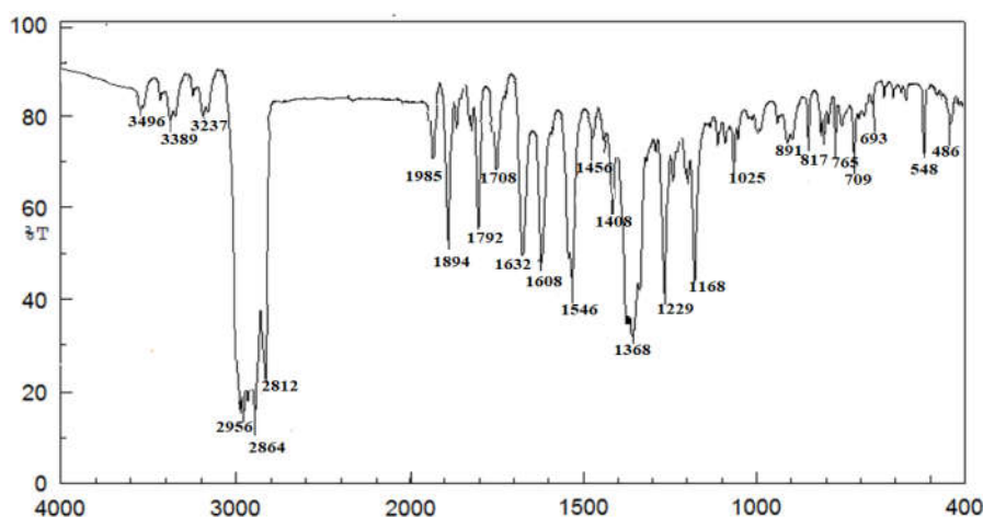
Fig 3. IR spectrum of the complex compound [\text{Co}(\text{2-hnaph})_2(\text{1,2-phen})_2]\cdot\text{Cl}\cdot\text{C}_2\text{H}_5\text{OH} .
