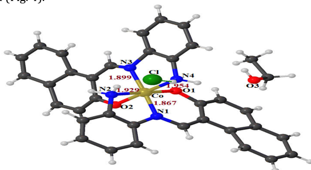
Fig 4. Molecular structure of the complex [\text{Co}(\text{2-hnaph})_2(\text{1,2-phen})_2]\cdot\text{Cl}\cdot\text{C}_2\text{H}_5\text{OH}
