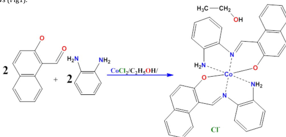
Fig 1. Synthesis scheme of the complex [\text{Co}(\text{2-hnaph})_2(\text{1,2-phen})_2]\cdot\text{Cl}\cdot\text{C}_2\text{H}_5\text{OH}
