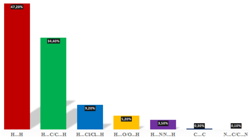
Fig 6. Hirshfeld fingerprint diagram of the complex with the composition [\text{Co}(\text{2-hnaph})_2(\text{1,2-phen})_2] \cdot \text{Cl} \cdot \text{C}_2\text{H}_5\text{OH}
