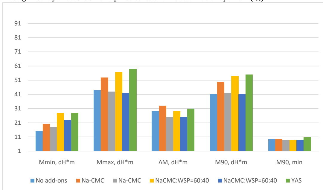
Figure 1. Rheometric properties of rubber compounds, %
