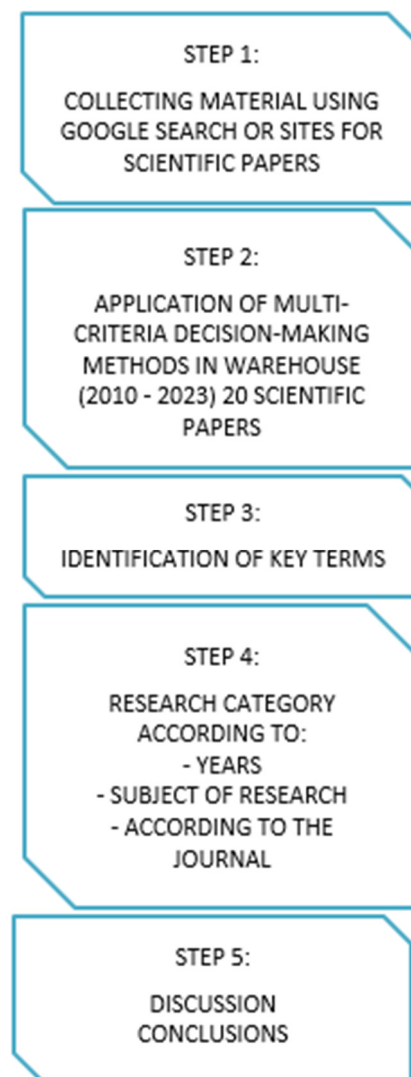
Fig. 1. Methodology
